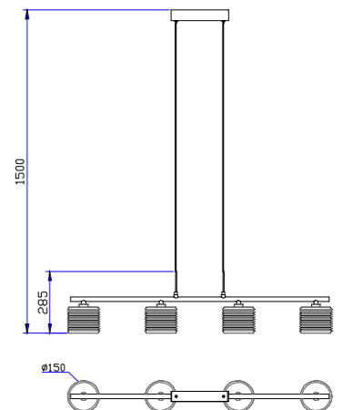
P0767-4A 20W 1230*285*150MM(1500mm)
