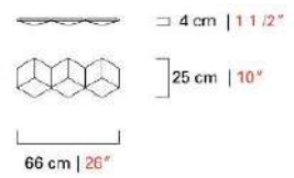
7253W/3 L660*E40*H250mm
