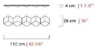
7253W/5 L1100*E40*H250mm
