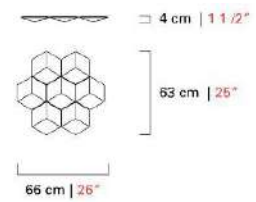
7253W/7 L660*E40*H630mm
