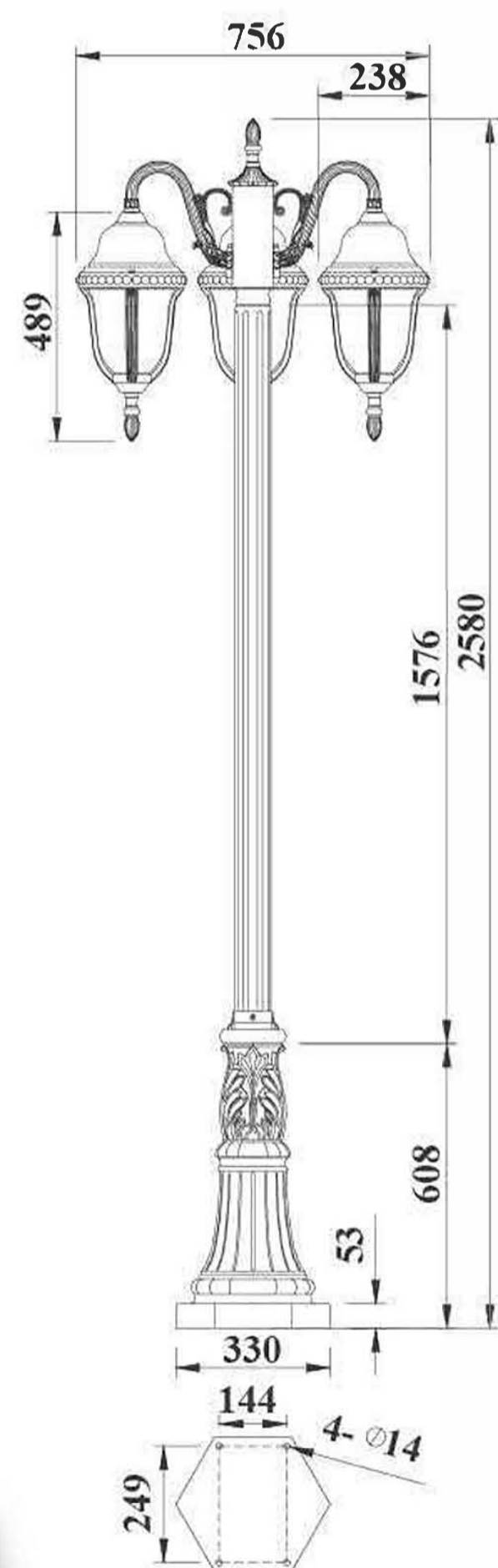
(Unit: mm) Color: 21# Glass: clear line glass Bulb: 3*100W E27 or E26 Material: Aluminum
