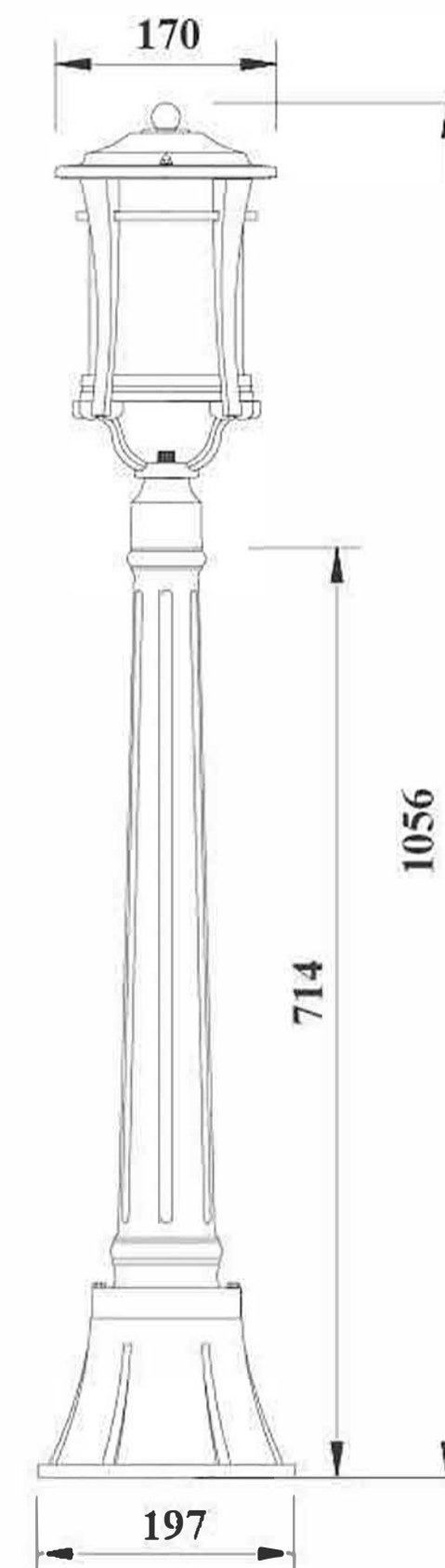
(Unit: mm) Color: 02# Glass: opal glass Bulb: 1*100W E27 or E26 Material: Aluminum
