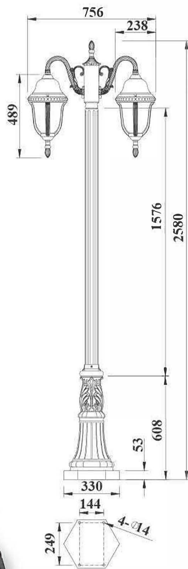
(Unit: mm) Color: 21# Glass: clear line glass Bulb: 2*100W E27 or E26 Material: Aluminum
