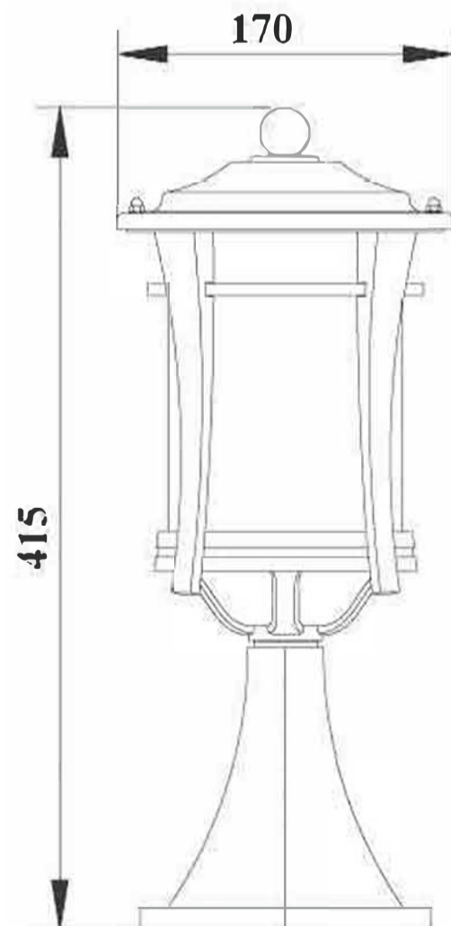
(Unit: mm) Color: 02# Glass: opal glass Bulb: 1*100W E27 or E26 Material: Aluminum
