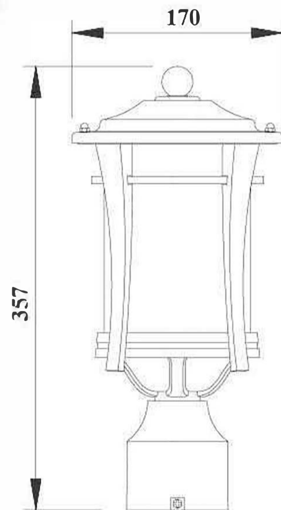
(Unit: mm) Color: 02# Glass: opal glass Bulb: 1*100W E27 or E26 Material: Aluminum
