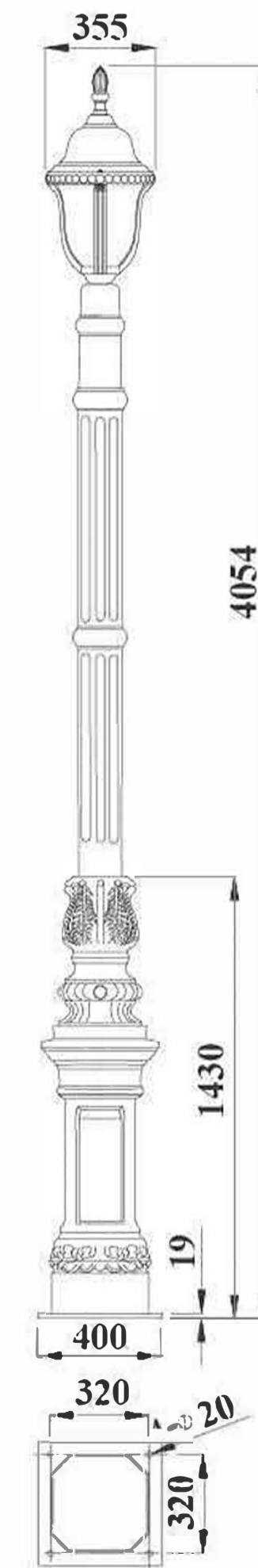
(Unit: mm) Color: 161# Glass: clear line glass Bulb: 1*100W E27 or E26 Material: Aluminum
