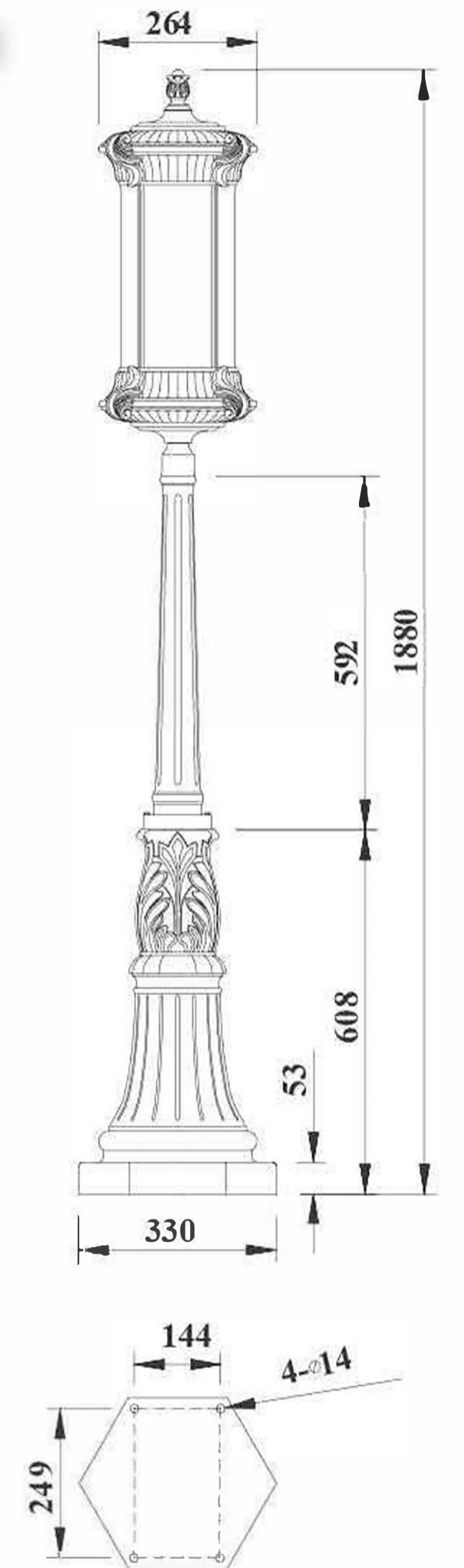
(Unit: mm) Color: 46# Glass: seedy glass Bulb: 3*60W E12 or E14 Material: Aluminum
