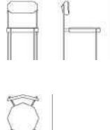
TYPE C348- Dining chair SIZE I 450WX560DX830H
