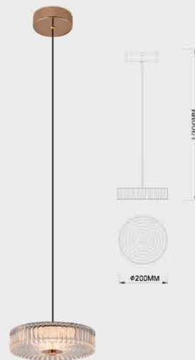
F-PP-D0820-φ200
