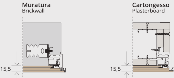
Muratura Brickwall
