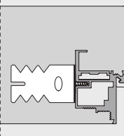
Muratura Brickwall
