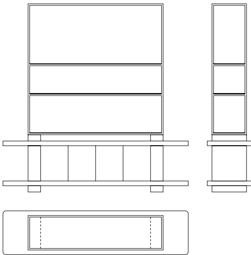
bookshelf n°1 with 4 doors— GSMA733 cm 236 x 56 | h. cm 240
