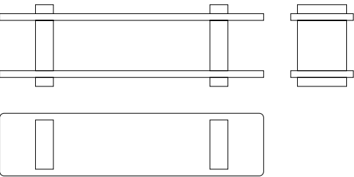
sideboard — GSMA931 cm 236 x 56 | h. cm 73
