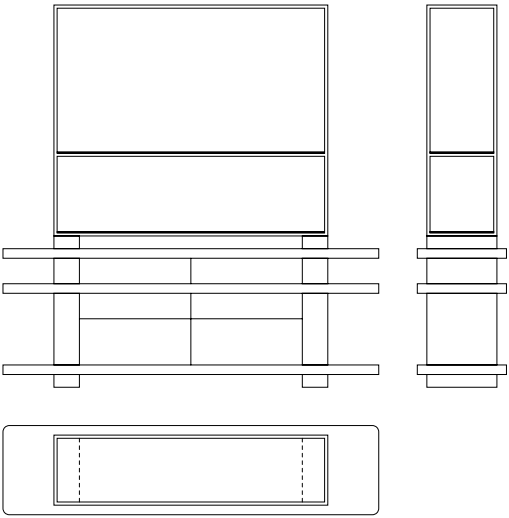
bookshelf n°2 with 6 drawers — GSMA834 cm 236 x 56 | h. cm 240
