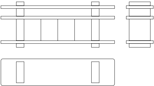
console with 4 doors — GSMC633 cm 236 x 56 | h. cm 95
