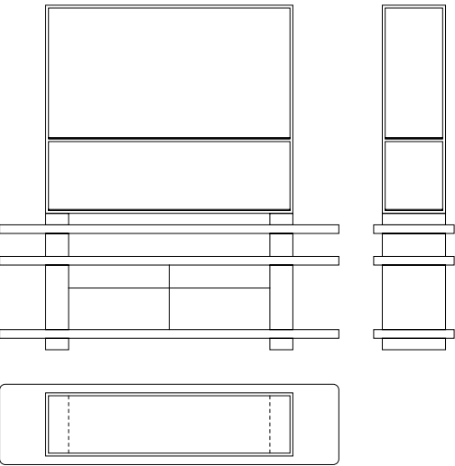
bookshelf n°2 with 4 drawers — GSMA832 cm 236 x 56 | h. cm 240
