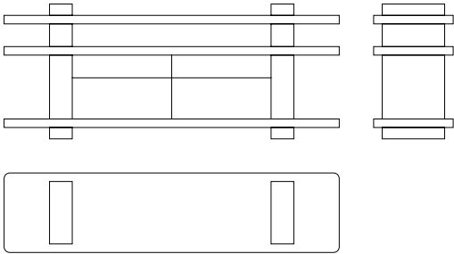
console with 4 drawers — GSMC632 cm 236 x 56 | h. cm 95
