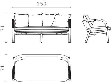
JISELLE love seat
