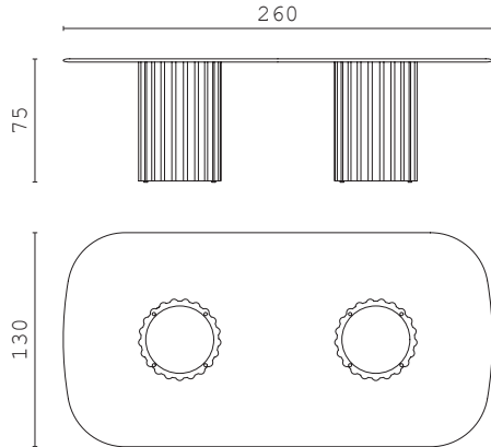
PABLO rectangular table
