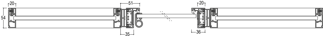
Stipite Cube abbinato a porta a battente Vitra e vetrate fisse _Cube frame combined with Vitra Hinged door and fixed glass panels
