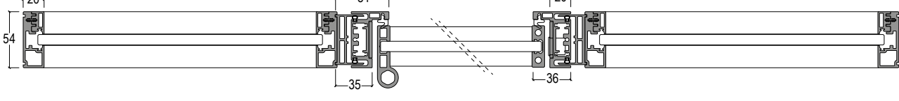
Stipite Cube abbinato a porta a battente 180 e vetrate fisse _Cube frame combined with Hinged door 180 and fixed glass panels
