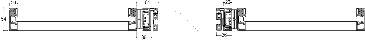
Stipite Cube abbinato a porta a battente Manhattan e vetrate fisse _Cube frame combined with Manhattan Hinged door and fixed glass panels
