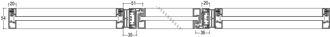
Stipite Cube abbinato a porta a bilico e vetrate fisse _Cube frame combined with Pivot door and fixed glass panels
