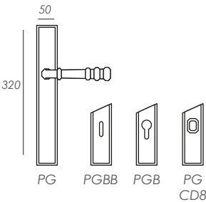
Rectangular Backplate Placa Rectangular
