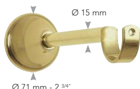
Platine 4 points 4 points plate
