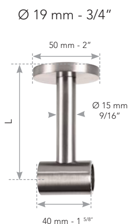
Platine 3 points 3 points plate
