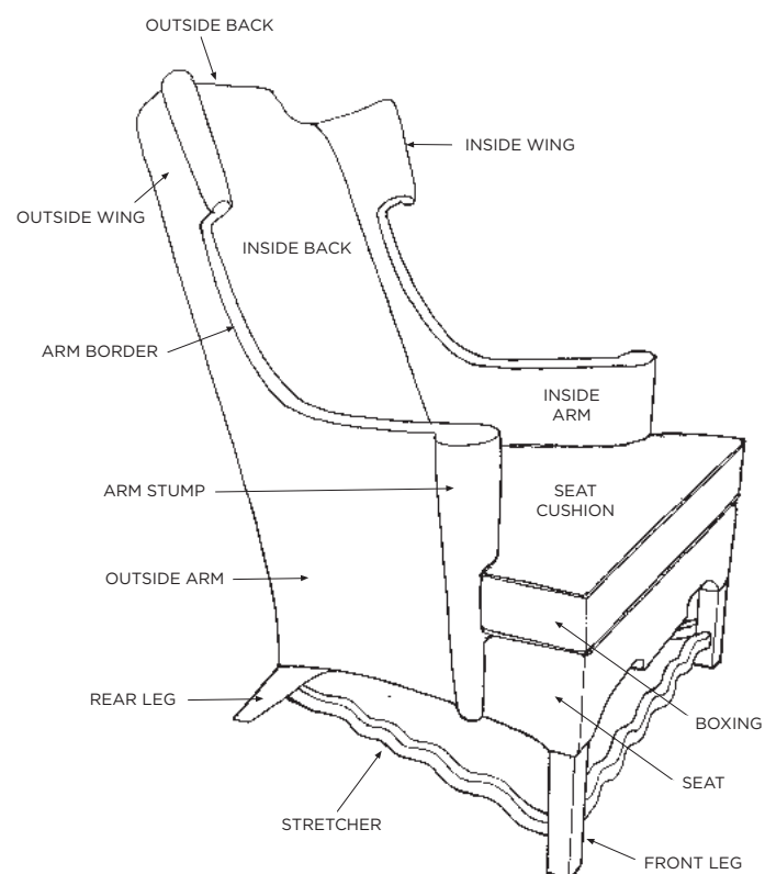
BASIC CHAIR PARTS - EXTERIOR
