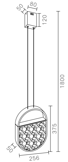
MD1851B-2A Stainless steel + Spanish alabaster /PC 28W
