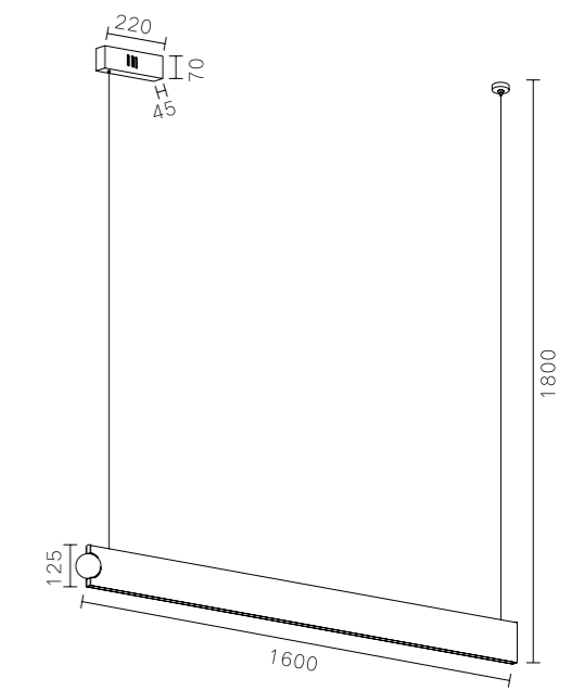
MD1835B-16A Stainless steel + PC 70W
