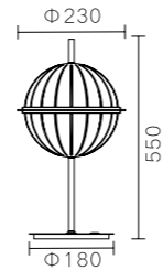
MT1924A-1A Stainless steel + Acrylic 12W
