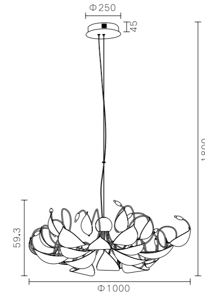
MD0266A-12A Stainless steel 12*2W
