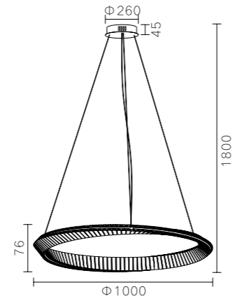
MB6080B-1A Stainless steel++Crystal 22W
