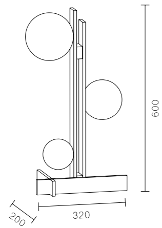
MT1508B-3A Stainless steel + Glass 8W
