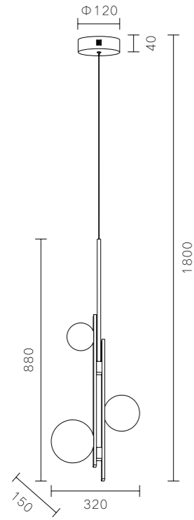
MD1508A-3A Stainless steel + Glass 8W
