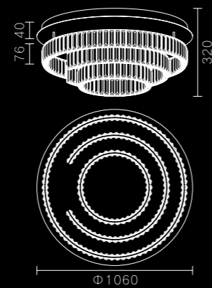
MX6063A-10A LED:3014#90W Size:φ1060*H320
