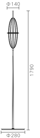
ML1925A-1A Stainless steel + Acrylic 8W
