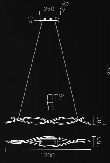
MD1844A-12A Stainless steel + PC 28W
