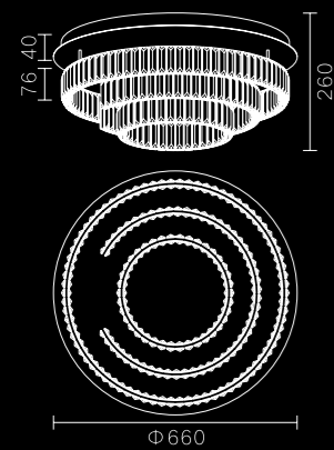
MX6063A-6A LED:3014#40W Size:φ660*H260
