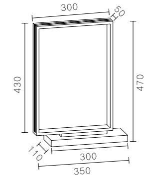
MT1550A-4A Stainless steel + PC 15W
