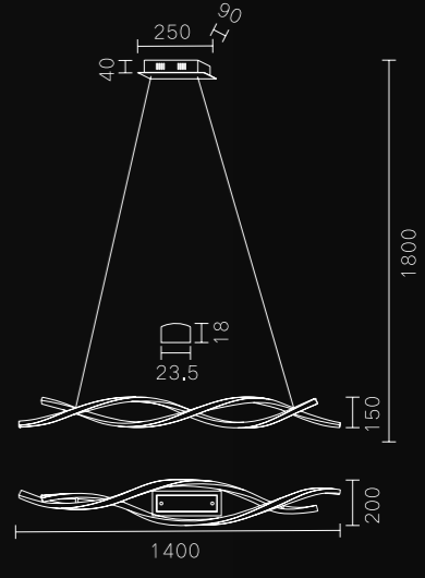
MD1844B-14A Stainless steel + PC 33W
