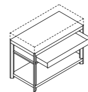
free-standing washstand (h 27 1/2" and 33 1/2") w 21 5/8", 27 1/2", 33 1/2", 39 3/8", 45 1/4", 51"
