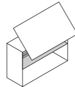
1 flap door, 1 shelf w 23 5/8", 29 1/2", 35 1/2", 41 1/4", 47 1/4"
