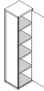
1 door, 5 shelves w 15 3/4", 21 5/8"
