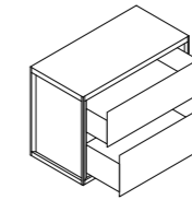
2 drawers (h 33 1/2") w 18", 23 5/8", 29 1/2", 35 1/2", 41 1/4", 47 1/4"
