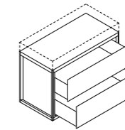
2 drawers w 18", 23 5/8", 29 1/2", 35 1/2", 41 1/4", 47 1/4"
