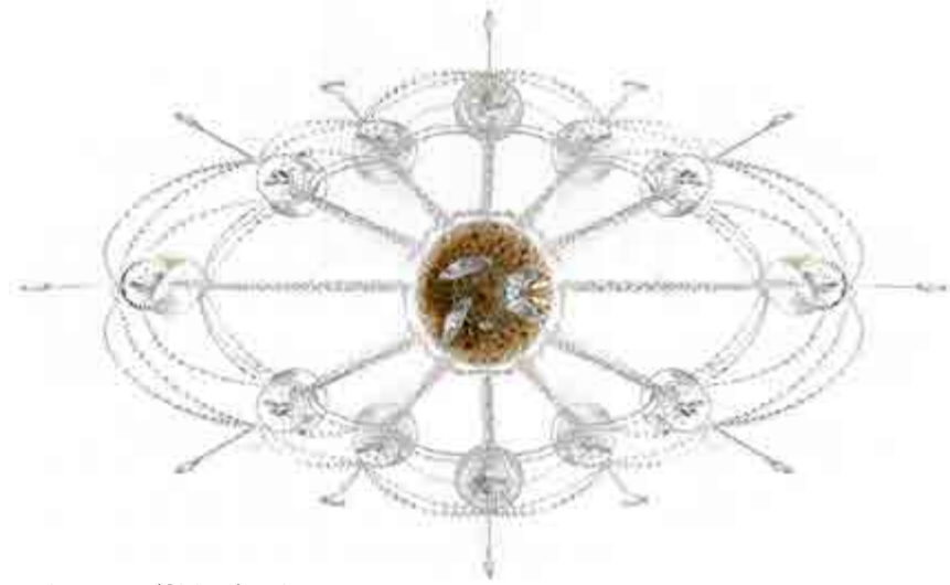
Art. 1761/CH12/ovale L 165 x 95 cm H 115 cm Pø 16 cm 12 x E14 x 40W
