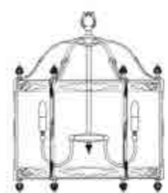
Art.1881/P ø 63 cm H 76 cm 6 x E27 x 40W
