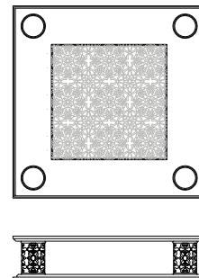
AT 622 SARAYA TAVOLINO CON TOP IN LEGNO E VETRO INCISO DECORO STELLA SIDE-TABLE WITH WOODEN TOP AND DECORATED GLASS CM 150X150XH40
