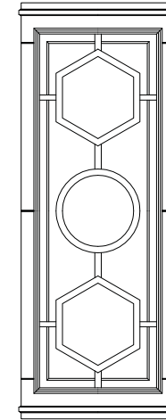
AP 901 CAESAR PANNELLI DECORATIVI DECORATIVE PANELS CM 121XH327,5
