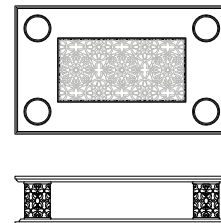
AT 624 SARAYA TAVOLINO CON TOP IN LEGNO E VETRO INCISO SIDE-TABLE WITH WOODEN TOP AND DECORATED GLASS CM 90X150XH40
