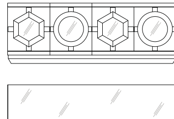
C 904 CAESAR CREDENZA 4 ANTE 4 DOORS SIDEBOARD CM 241X50XH84,5
