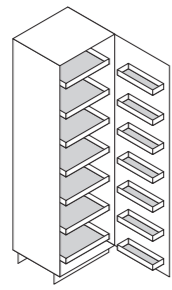
1 door w/sliding trays w 12", 18", 23 5/8"
