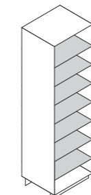
1 open-faced unit w 5 7/8" - 23 5/8"
