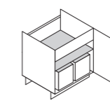
sink unit, 1 heavy-duty drawer with built-in waste bins w 18", 23 5/8", 35 1/2", 47 1/4"
