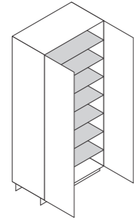
2 doors, shelves w 35 7/8"
