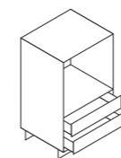
1 oven unit, 2 drawers w 23 5/8", 30", 36"
