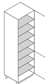
2 doors, shelves w 12", 18", 23 5/8"
