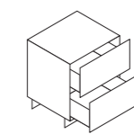
2 heavy-duty drawers w 18", 23 5/8", 35 7/8", 47 1/4"
